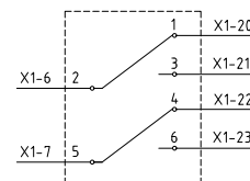
PRESSURE SAFETY DEVICE
