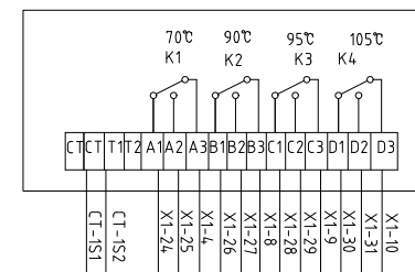
Winding thermometerBWR-4
