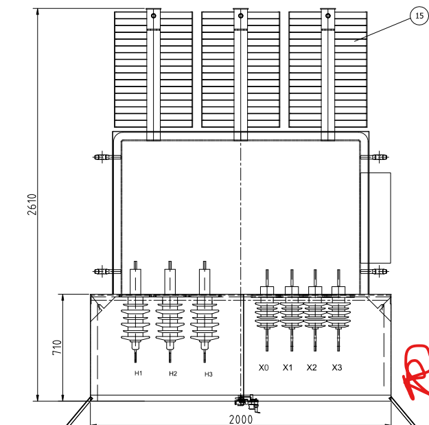
REMOVEABLE GLAND PLATE
